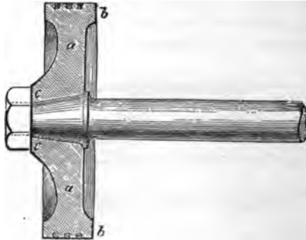
FIG. 326.—The Piston of a small double-acting steam engine, showing method of connecting the piston rod, and the position of the packing rings. The parts are: a, a , the body of the piston; b, b , the circumference bearing the packing rings; c, c , the central boss receiving the coned end of the rod.
